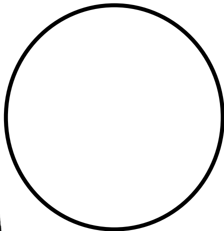
new moon
