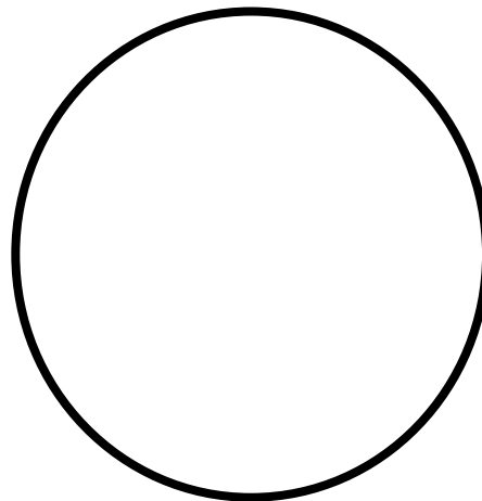
first quarter
