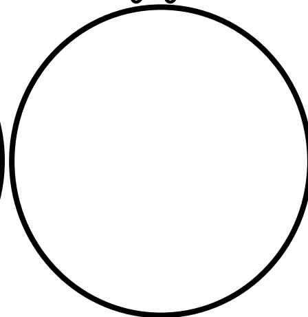
waning crescent
