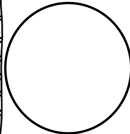
full moon
