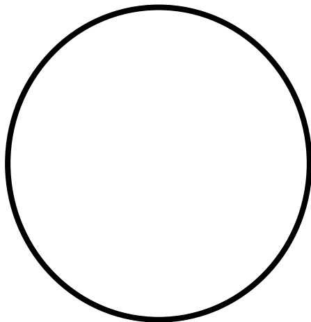
waxing crescent
